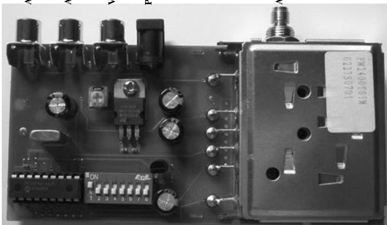
Freq. Setting by dipswitch*
